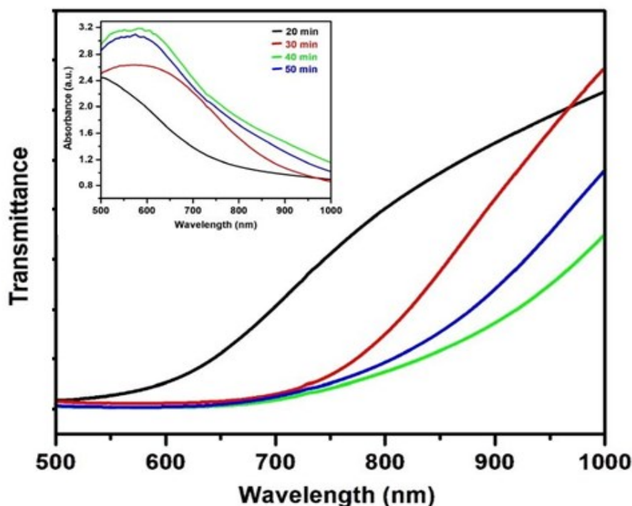
Fig. 9. Transmittance of nanocrystalline PbS thin films deposited on glass substrate at different deposition times. The inset shows the absorbance spectra obtained for the same thin films.
