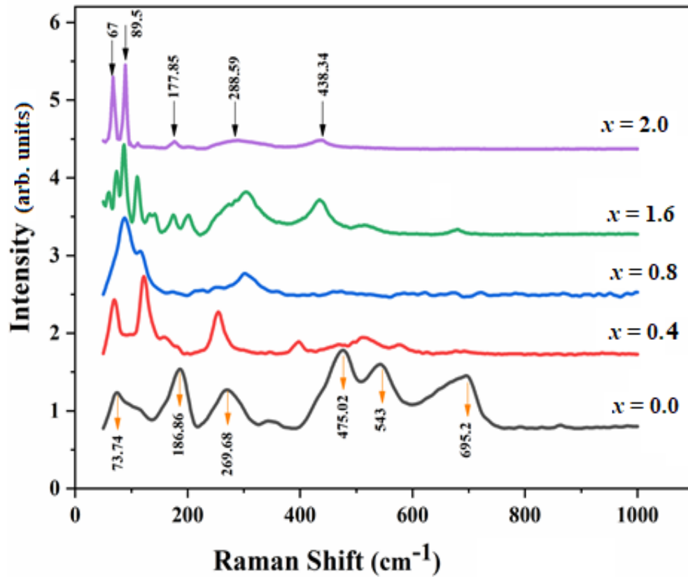
Fig. 3. Raman spectra of \text{CuFe}_{2-x}\text{Bi}_x\text{O}_4 ( x=0.0, 0.4, 0.8, 1.6 , and 2.0 )
