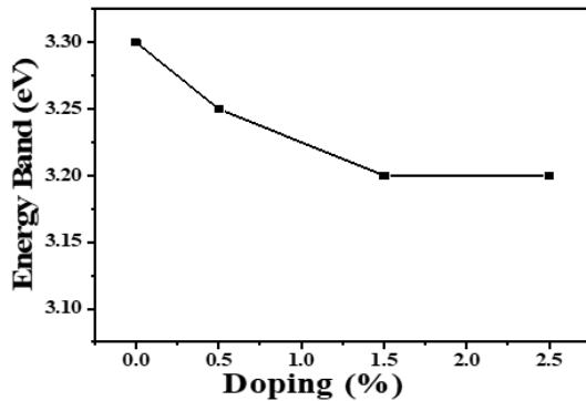
Fig. 7. Optical Bandgap Vs doping concentration
