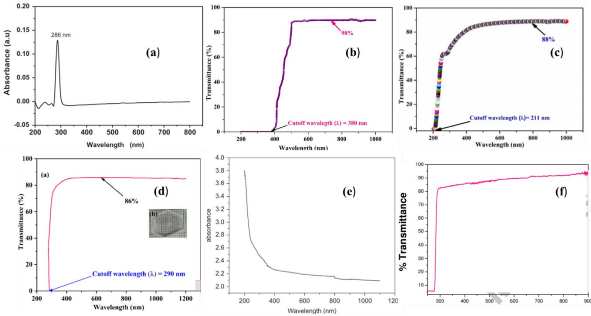
Fig. 1. shows the various NLO material UV-Visible NIR spectra.
